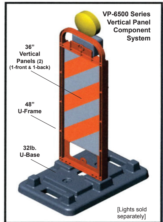
12"x36" reflective Vertical Panels on 48" U-Frame and 32 lb. U-Base (Panel-stripping available 12" x 24", 12" x 30", or 12" x 36"; stripes are EG, HI, or DG)
