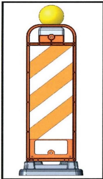
12"x36" reflective Vertical Panels on 48" U-Frame and 32 lb. U-Base (Panel-stripping available 12" x 24", 12" x 30", or 12" x 36"; stripes are EG, HI, or DG)
